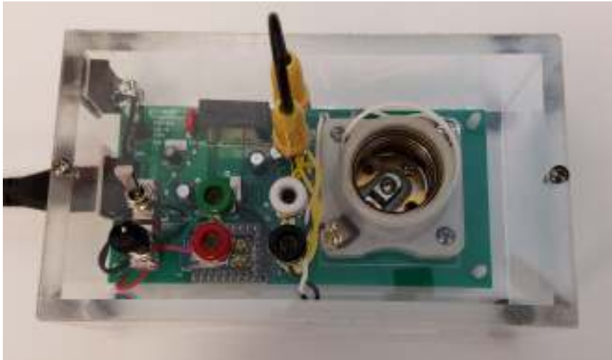
Figure 1 – Populated Circuit Board Photograph, Top.
