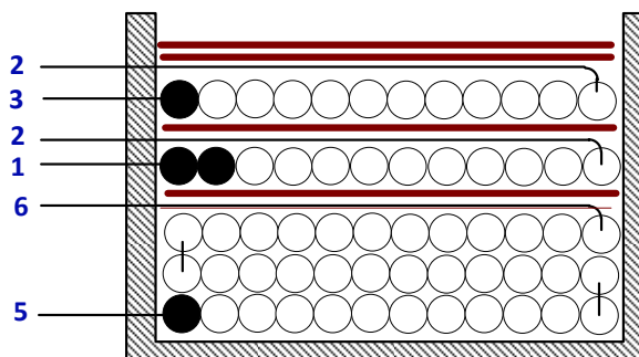
Figure 19 – Transformer Build Diagram.
