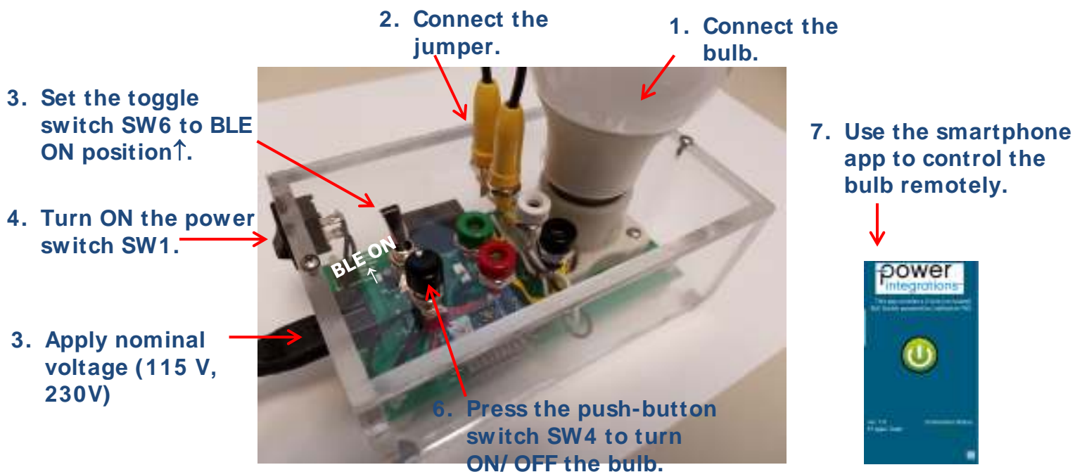
Figure 10 – Power-up Procedure.
